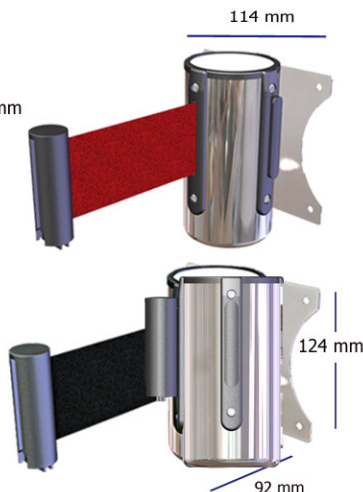
HWMPR/HWMPB: Wall Barrier Dimensions
